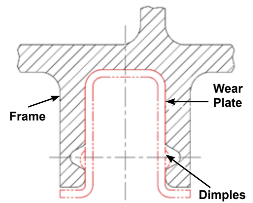
Captive Spring System
